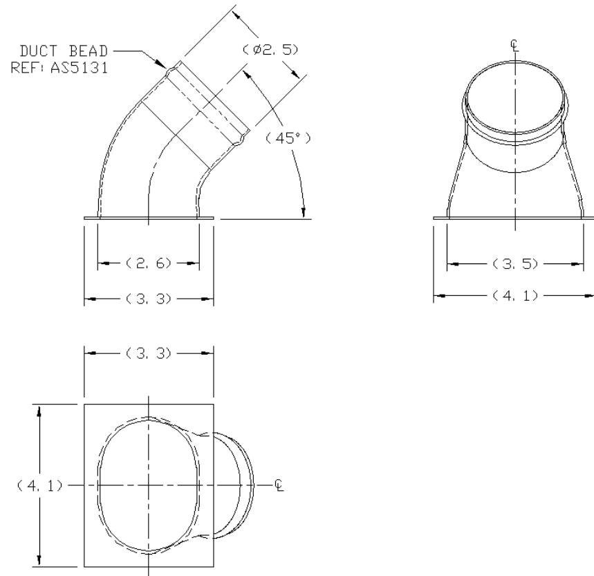
ANGLED STUB, 45° PART NO. JMIH-230-040-227 MATERIAL: KYDEX-100 OR FIBERGLASS
