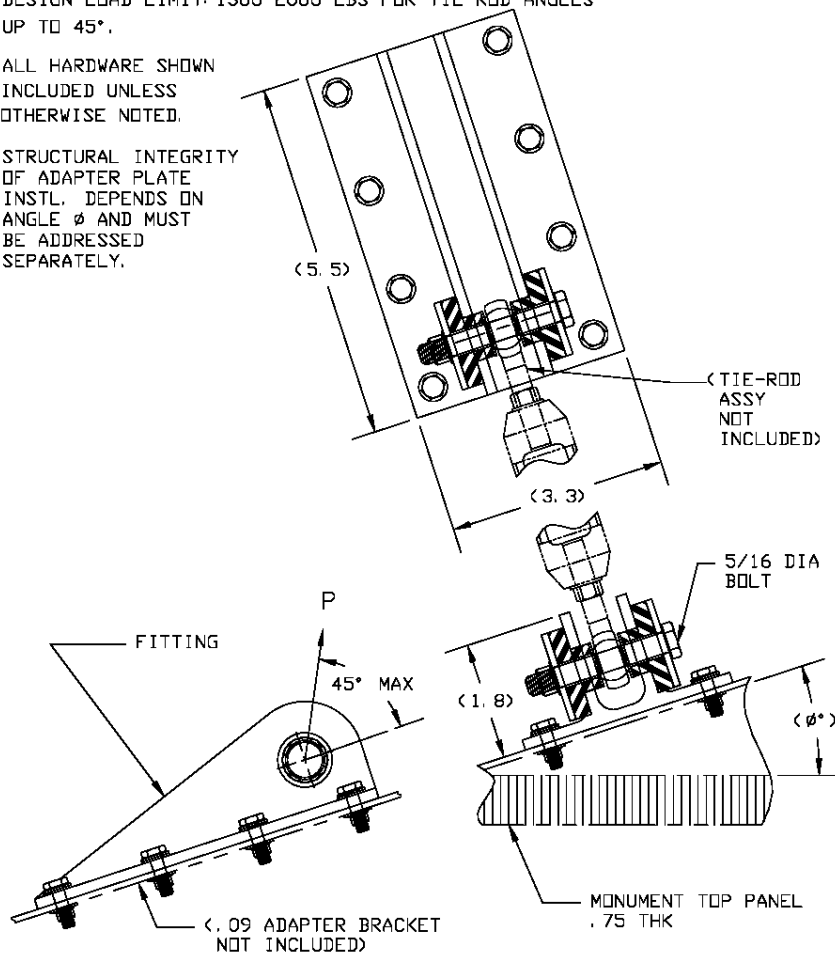
-025 MONUMENT FWD/AFT ATTACH, ADAPTER PANEL
