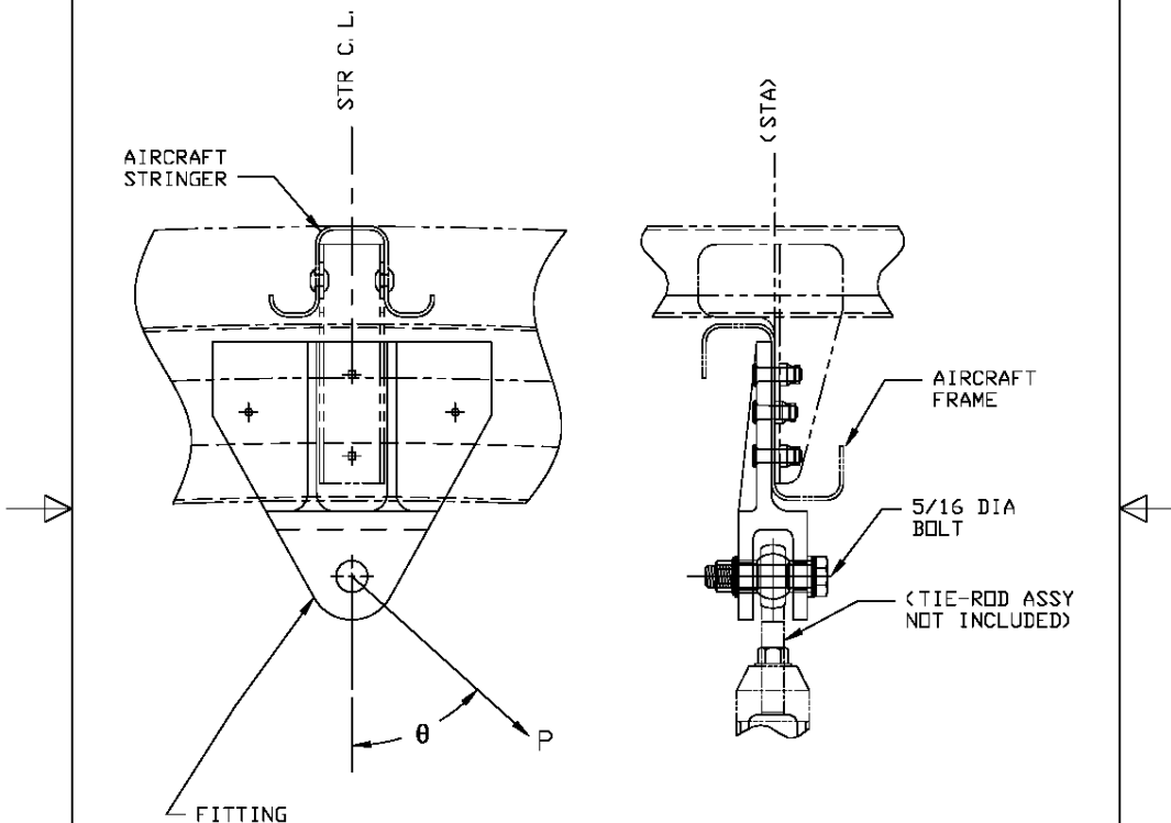
-017 FRAME ATTACHMENT, LATERAL
