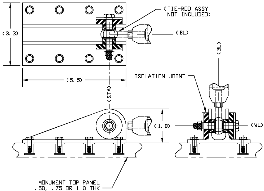
-005 MONUMENT FWD/AFT RESTRAINT
