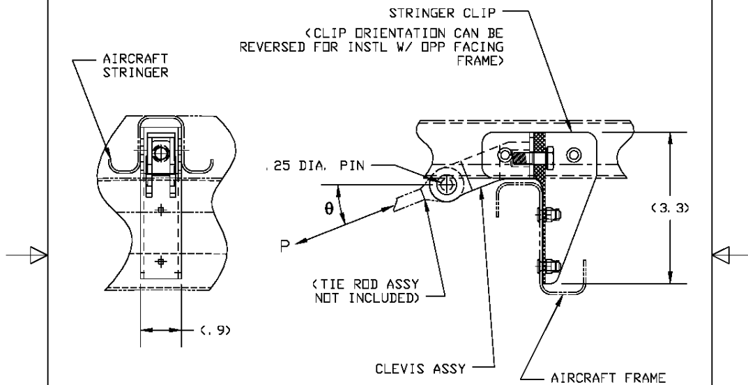
-015 STRINGER ATTACHMENT, FWD/AFT
