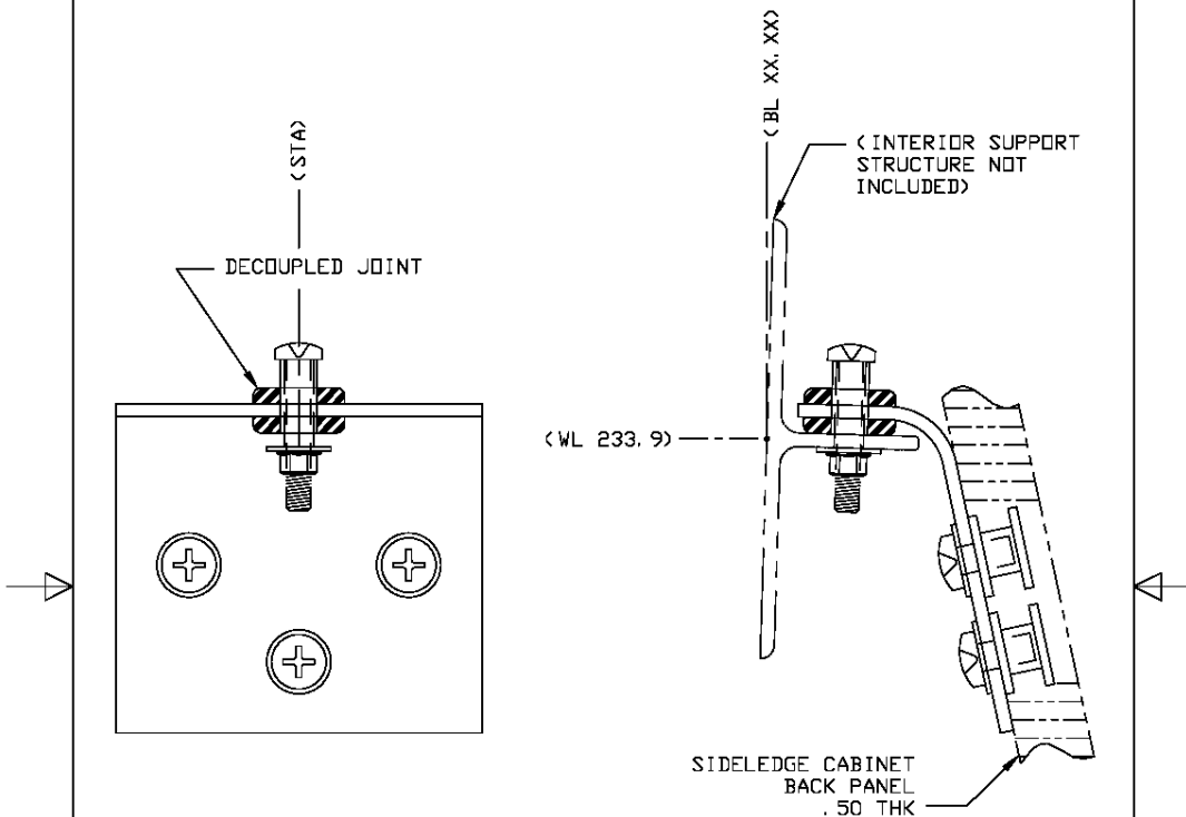
-013 UPPER SIDELEDGE ATTACHMENT, LWR.
